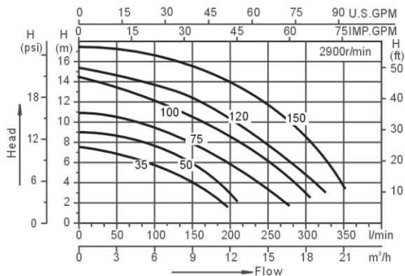
Performance Curves
